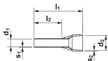
Figure 1 Dimensions (tolerances according to DIN 46228-4)
