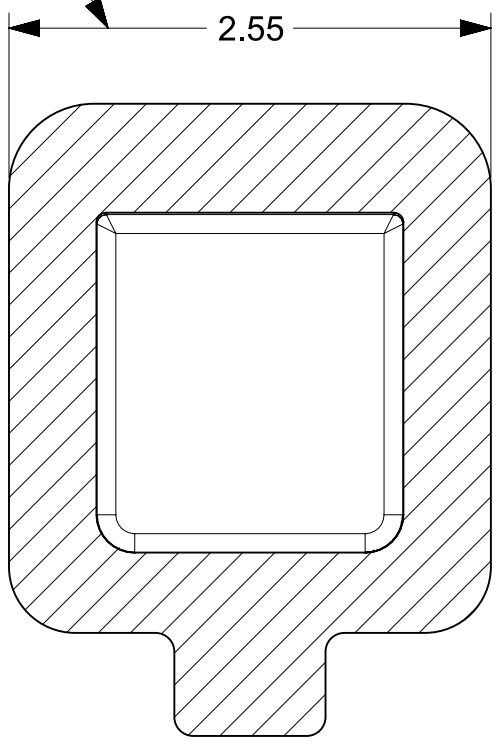
SECTION Z-Z
