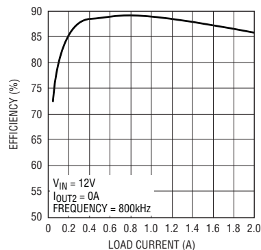
Switching Converter Efficiency
