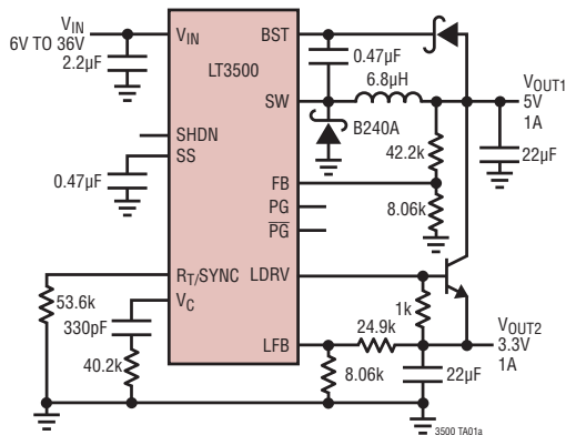
Dual Step-Down Converters
