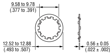
LOCKWASHER H-37-2
