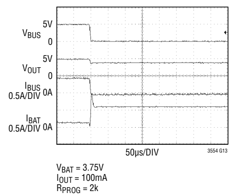
V BUS Disconnect Waveform
