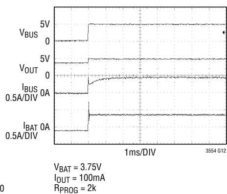
V BUS Connect Waveform
