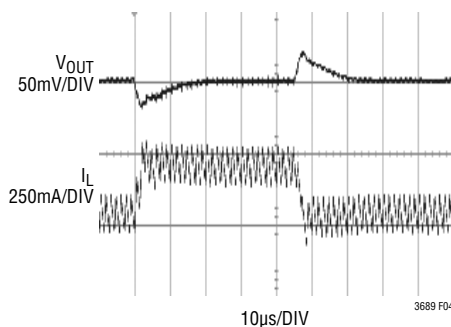
Figure 4. Transient Load Response of the LT3689 Front Page Application as the Load Current is Stepped from 360mA to 720mA. V_{OUT} = 3.3V , V_{IN} = 12V
