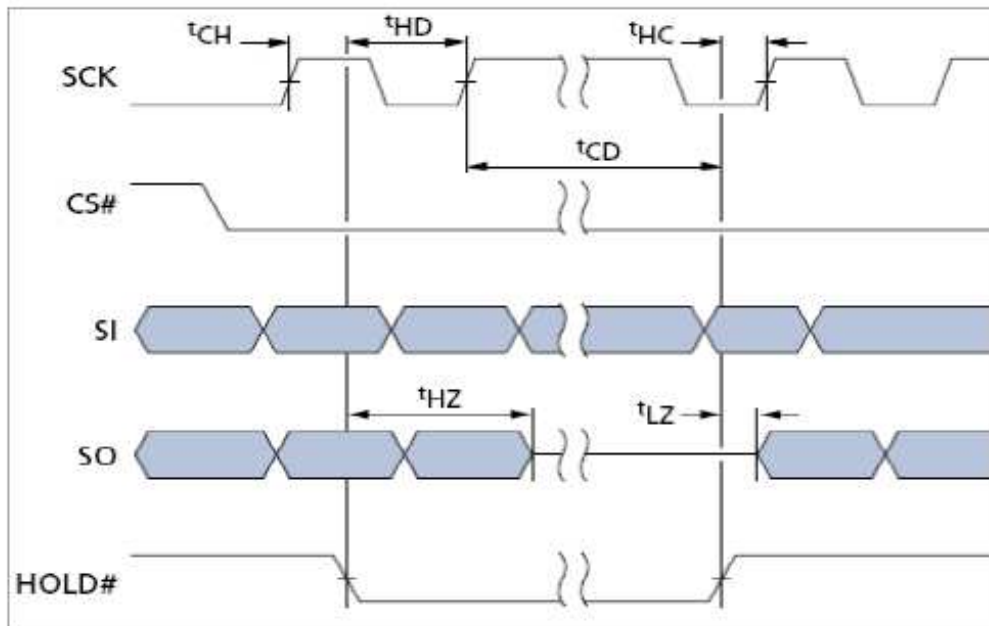
Figure 6.15 HOLD# Timing
