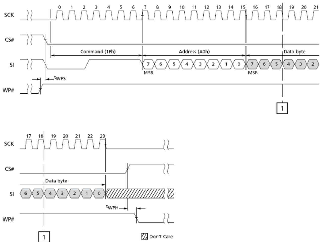
Figure 6.14 WP# Timing
