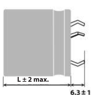
Four Pins 382L/LX (35, 40 and 45mm diameter)
