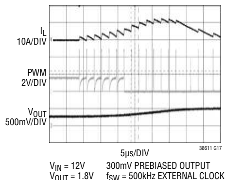
Initial 7-Cycle Nonsynchronous Start-Up (Single Phase Using FDMF6707B DrMOS)
