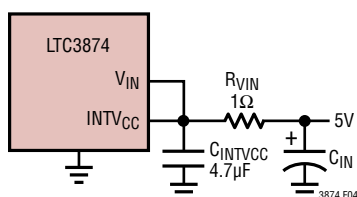
Figure 4. Setup for a 5V Input
