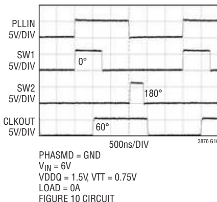
Phase Relationship: PHASMD = Ground (Forced Continuous Mode)
