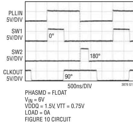
Phase Relationship: PHASMD = Float (Forced Continuous Mode)
