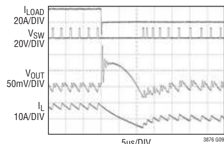
Load Release VTT
