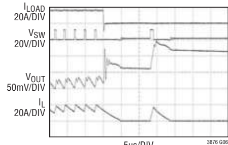
Load Release VDDQ (Discontinuous Mode)
