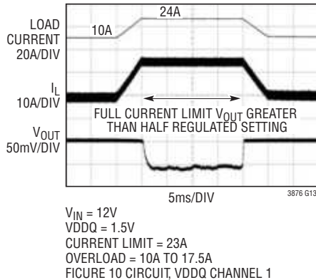
Overcurrent Protection (Forced Continuous Mode)
