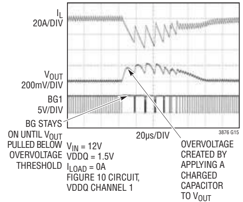
Overvoltage Protection (Forced Continuous Mode)
