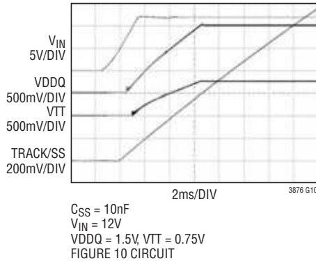
Regular Soft Start-Up (Forced Continuous Mode)
