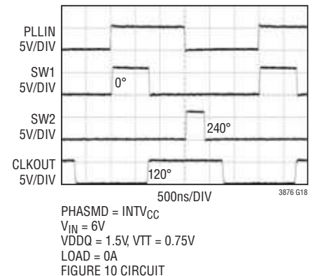
Phase Relationship: PHASMD = INTV CC (Forced Continuous Mode)
