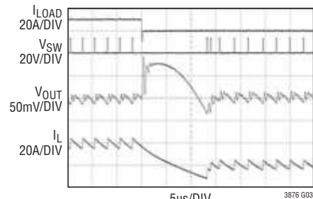
Load Release VDDQ (Forced Continuous Mode)
