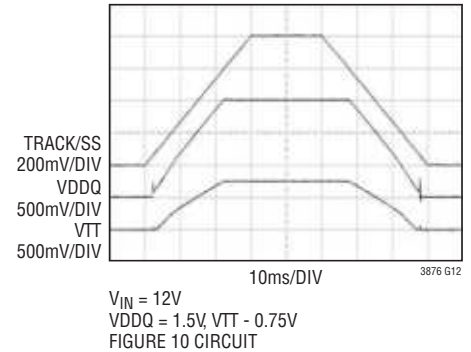
Output Tracking (Forced Continuous Mode)
