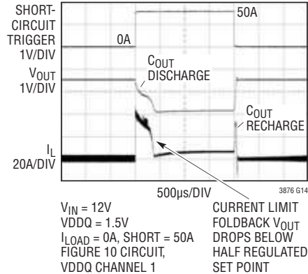
Short-Circuit Protection (Forced Continuous Mode)
