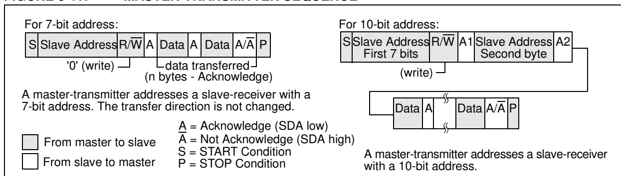
FIGURE 9-11: MASTER-TRANSMITTER SEQUENCE
