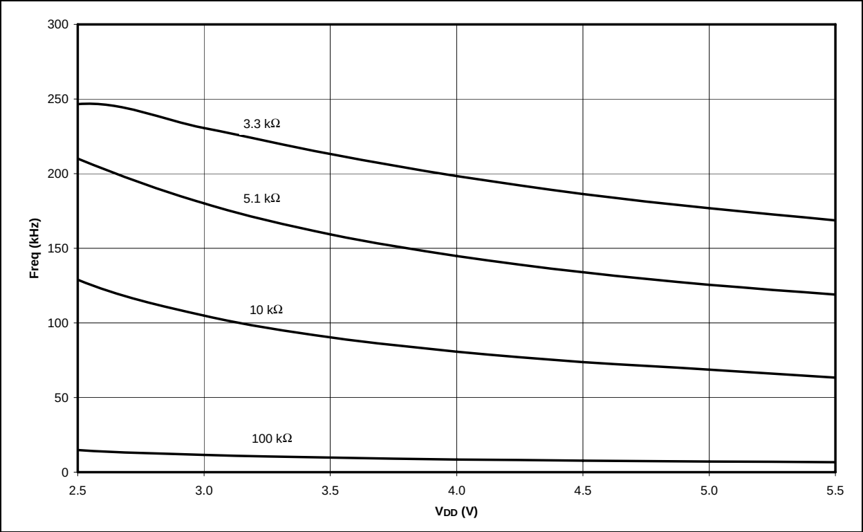
FIGURE 15-9: AVERAGE F_{osc} vs. V_{DD} FOR VARIOUS VALUES OF R (RC MODE, C = 300\text{ pF} , 25^\circ\text{C} )
