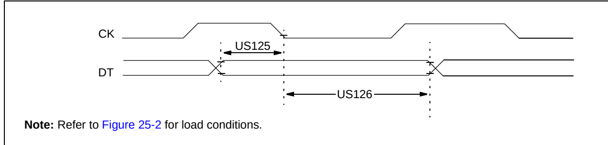
FIGURE 25-15: USART SYNCHRONOUS RECEIVE (MASTER/S�AVE) TIMING
