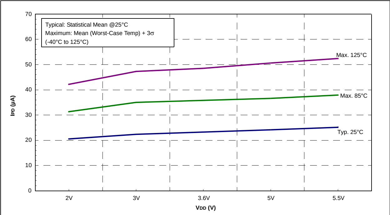
FIGURE 26-33: PIC16F707 BOR IPD vs. VDD, VCAP = 0.1μF
