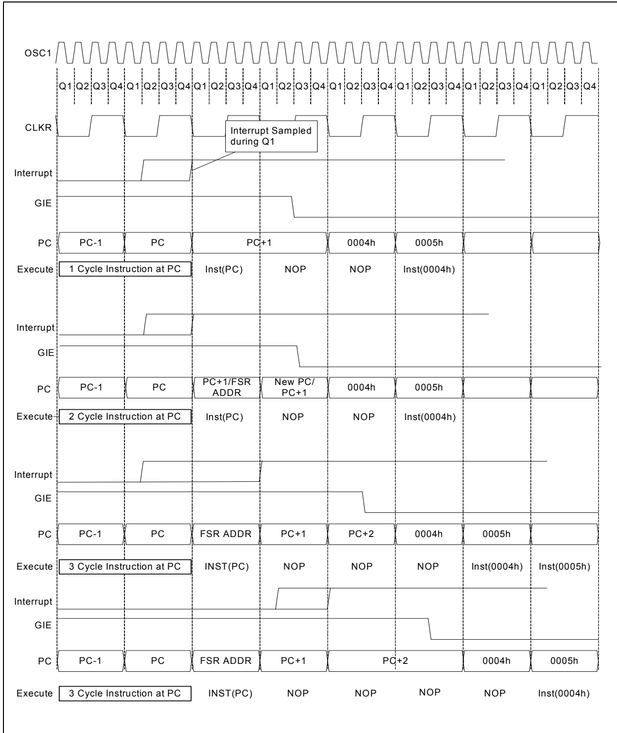
FIGURE 7-2: INTERRUPT LATENCY
