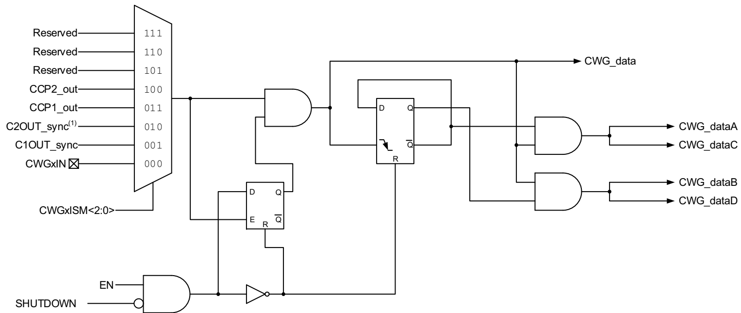
FIGURE 24-2: SIMPLIFIED CWG BLOCK DIAGRAM (PUSH-PULL MODE)
