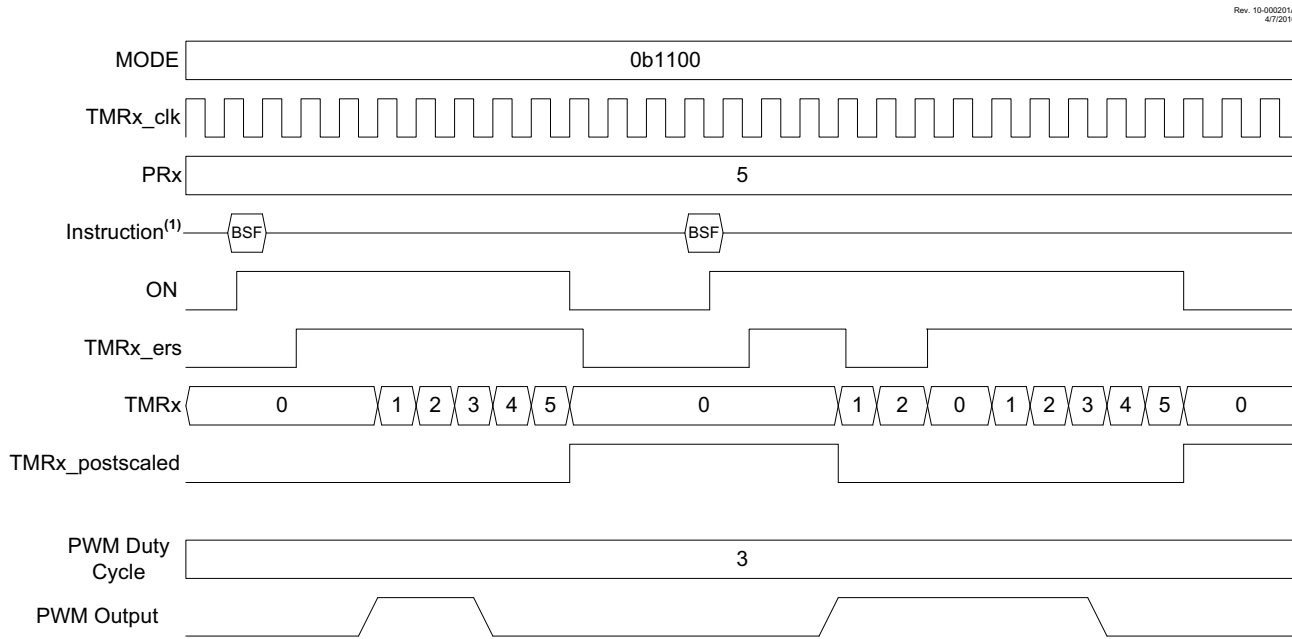
FIGURE 22-10: EDGE-TRIGGERED HARDWARE LIMIT ONE-SHOT TIMING DIAGRAM
