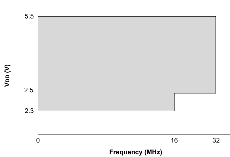
FIGURE 28-1: VOLTAGE FREQUENCY GRAPH, -40^{\circ}\text{C} \leq T_A \leq +125^{\circ}\text{C} , PIC12F1612/16F1613 ONLY
