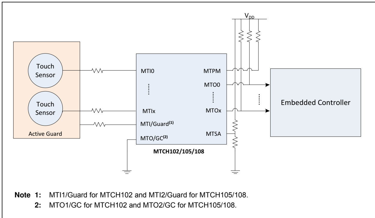
FIGURE 6: SYSTEM DIAGRAM FOR MTCH10X
