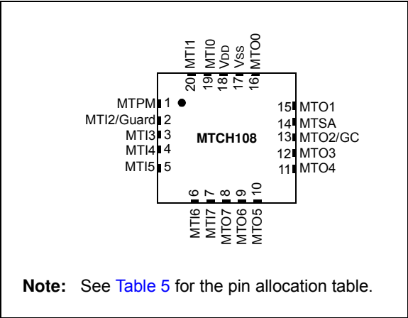
FIGURE 5: 20-LEAD QFN
