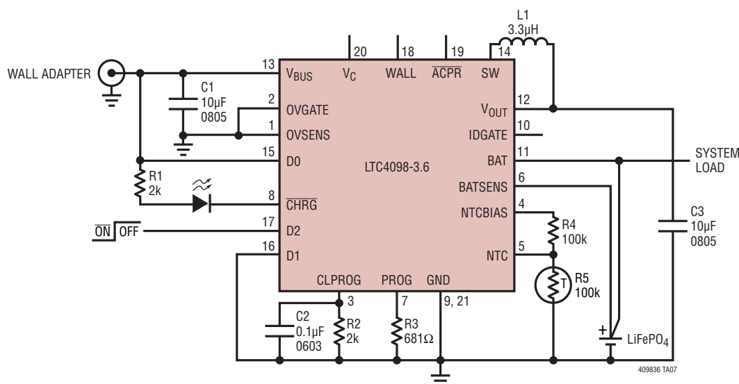
1.5A Standalone LiFePO 4 Charger
