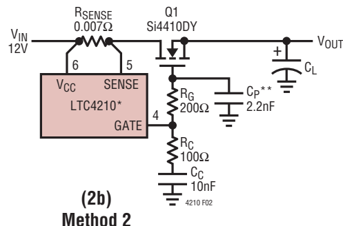
Figure 2. Frequency Compensation
