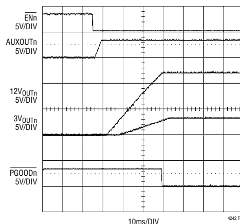
Normal Power-Up Sequence
