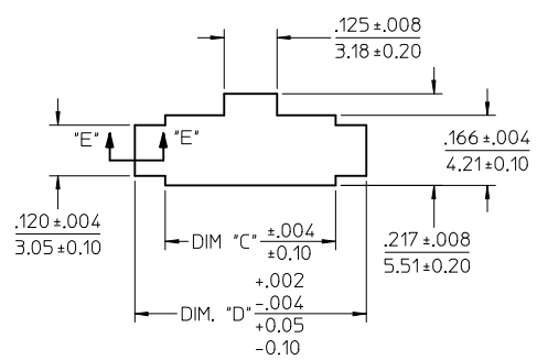
RECOMMENDED PANEL CUT-OUT (SEE NOTES 8 & 11)
