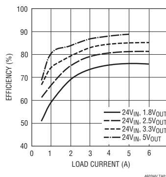
Efficiency vs Load Current with 24V IN
