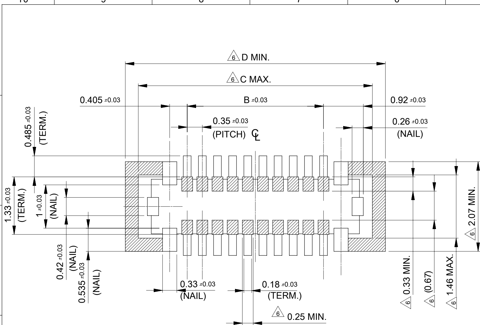
RECOMENDED P.W.BOARD PATTERN LAYOUT(REFFRENCE)
