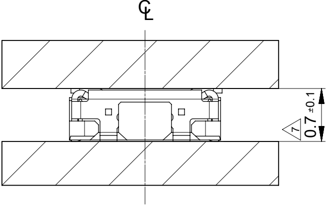
MATED CONDITION (505270/505070)
