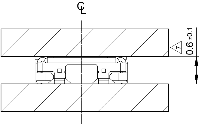
MATED CONDITION (505066/505070)
