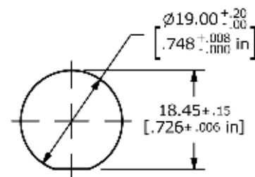
POWER SYMBOL PANEL CUTOUT
