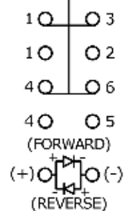
DPDT LED SCHEMATIC
