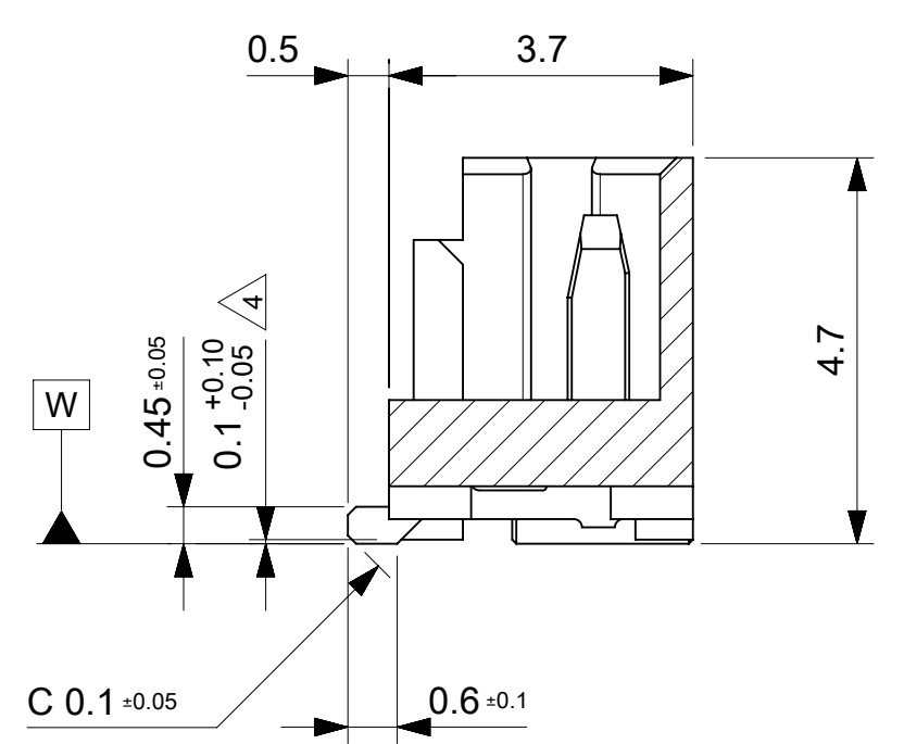
SECTION Z-Z
