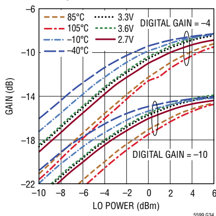
Gain vs LO Power at f_{LO} = 1260MHz
