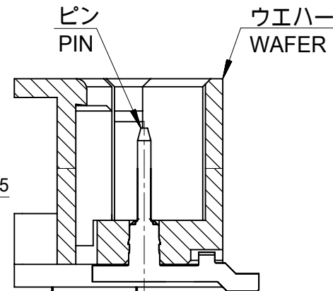
SECTION Z-Z
