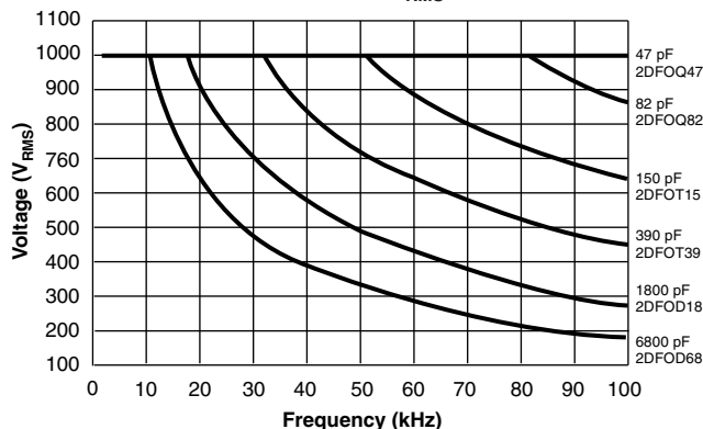
2DFO Series 1000 V RMS Low DF
