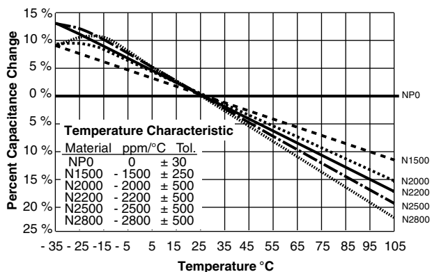
Temperature Characteristics for 1DFO, 2DFO &amp; 3DFO Series
