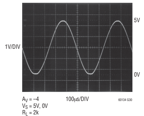
Rail-to-Rail Output Swing
