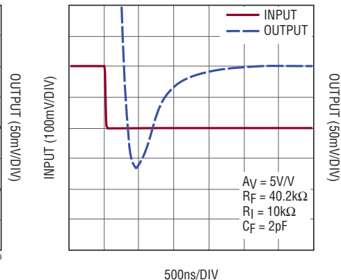
LTC6090-5 Falling Edge Settling Time
