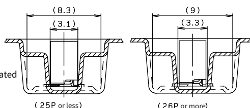
SECT. E-E
