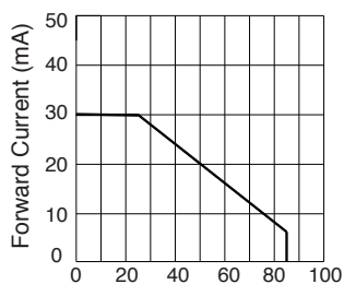
Forward Current vs. Derating Curve
