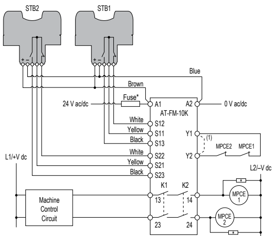
Connection to two STB Touch Buttons with contact outputs
