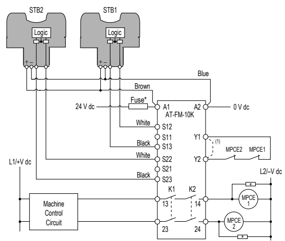
Connection to two STB Touch Buttons with PNP (sourcing) outputs
