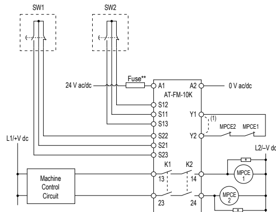
Connection to two mechanical push buttons with contact outputs
