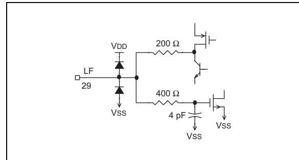
FIGURE 2-2: BLOCK DIAGRAM OF LOOP FILTER PIN
