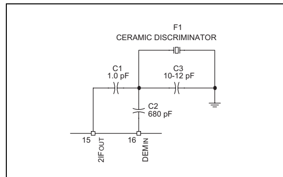
FIGURE 3-15: CERAMIC DISCRIMINATOR EXAMPLE CIRCUIT
