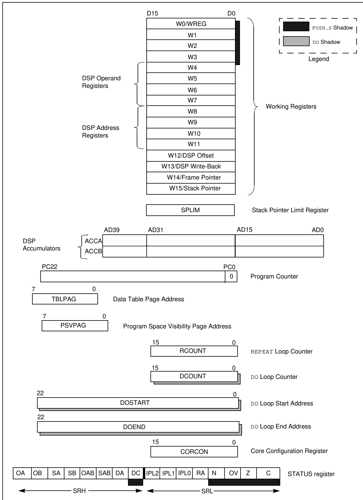
FIGURE 2-1: PROGRAMMER'S MODEL
