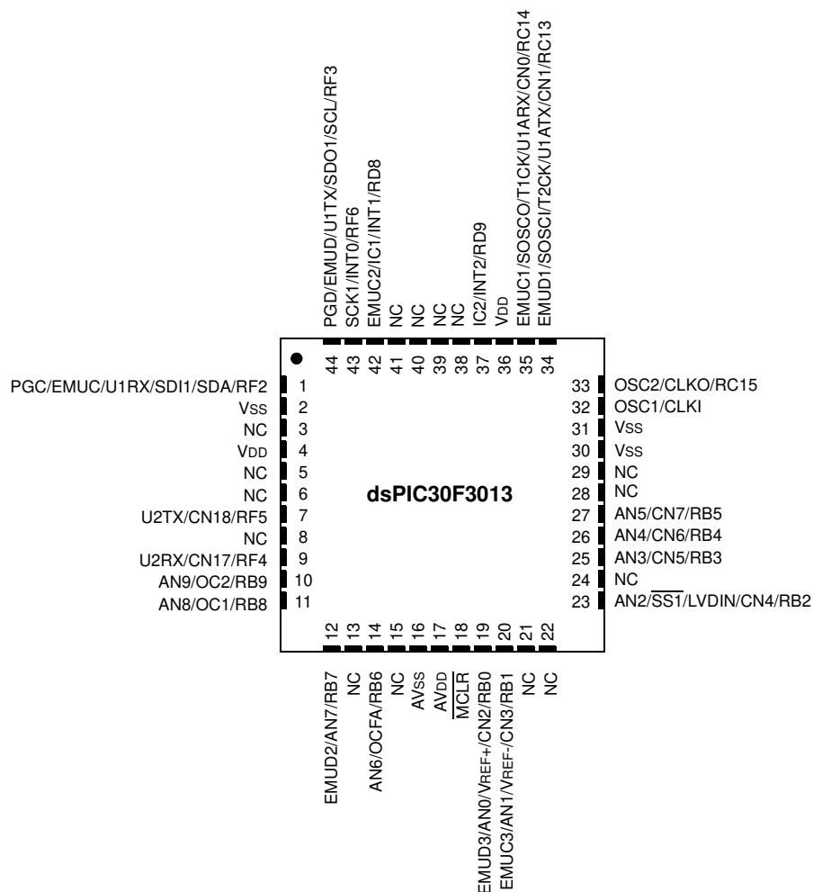
44-Pin QFN (1)
