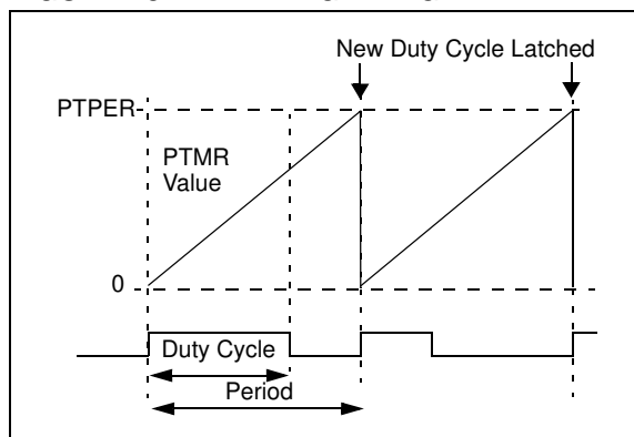
FIGURE 15-2: EDGE-ALIGNED PWM
