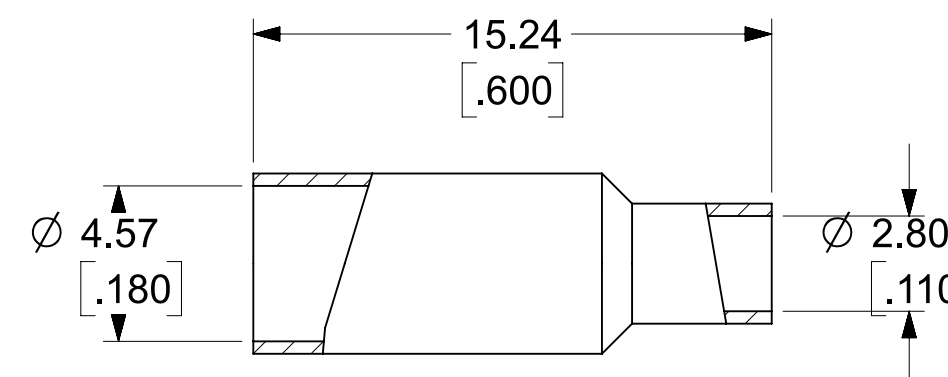
CRIMP TUBE
