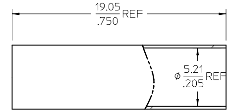
VERSAFIT SHRINK TUBE (SEE TABLE)
