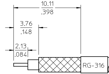
CABLE STRIP DIMENSIONS
