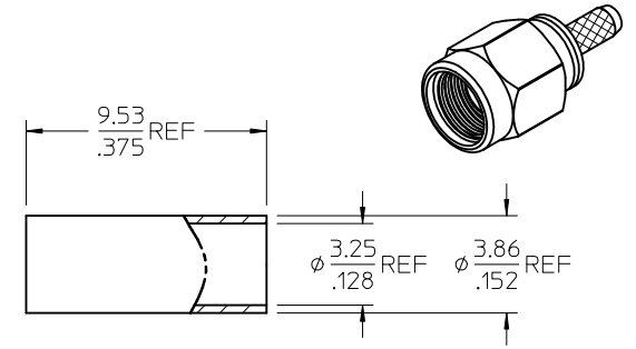
CRIMP TUBE
