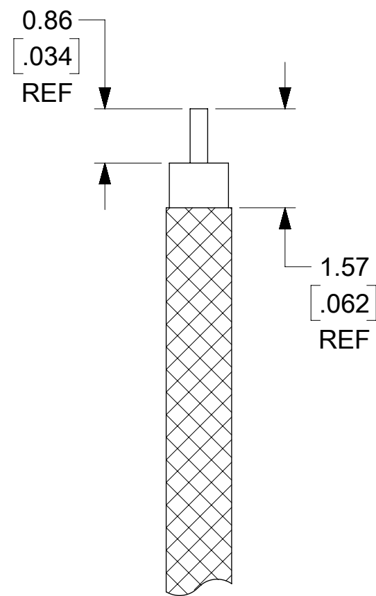
CABLE STRIP DIMENSIONS FOR NON-JACKETED CABLES
