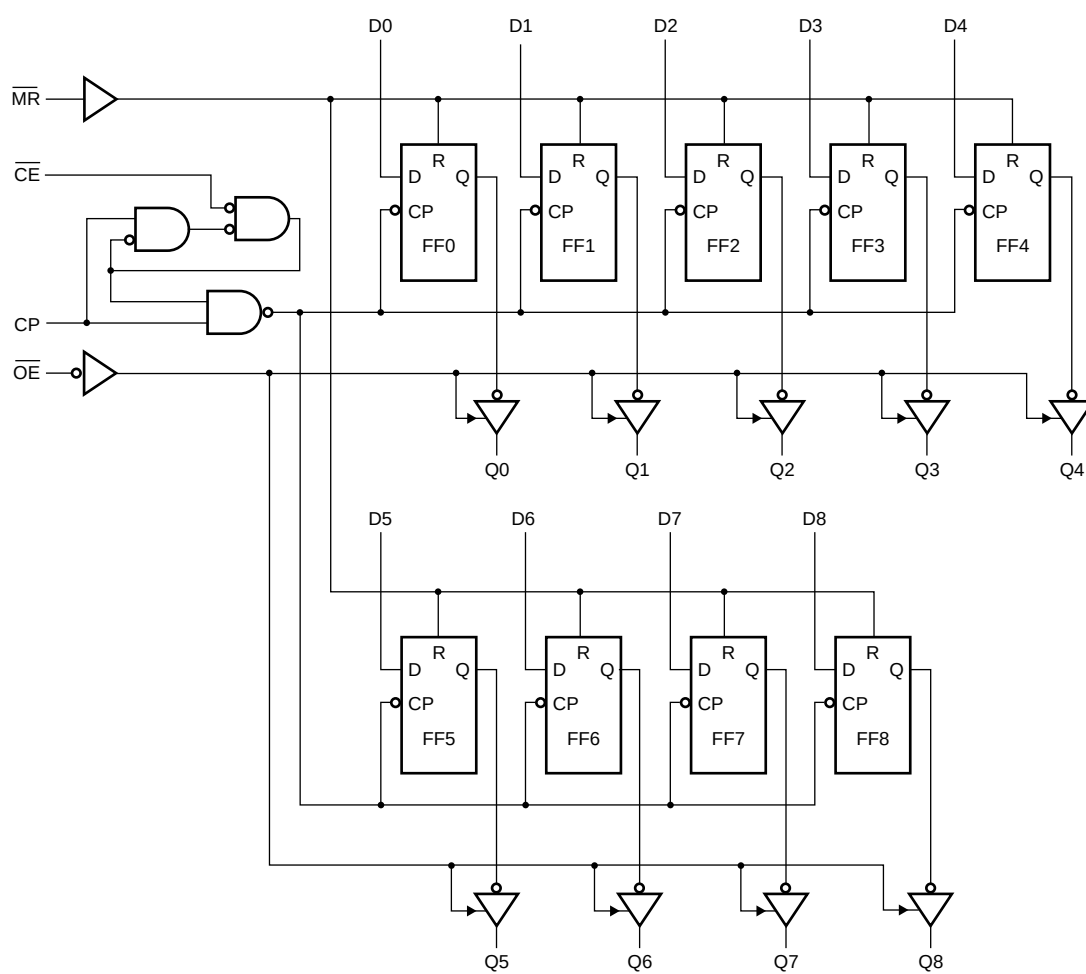
Fig 3. Logic diagram
