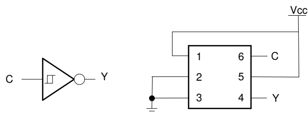
Configuration 6 Inverter
