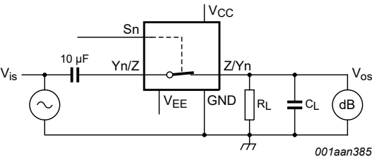
Fig. 14. Test circuit for measuring sine-wave distortion
