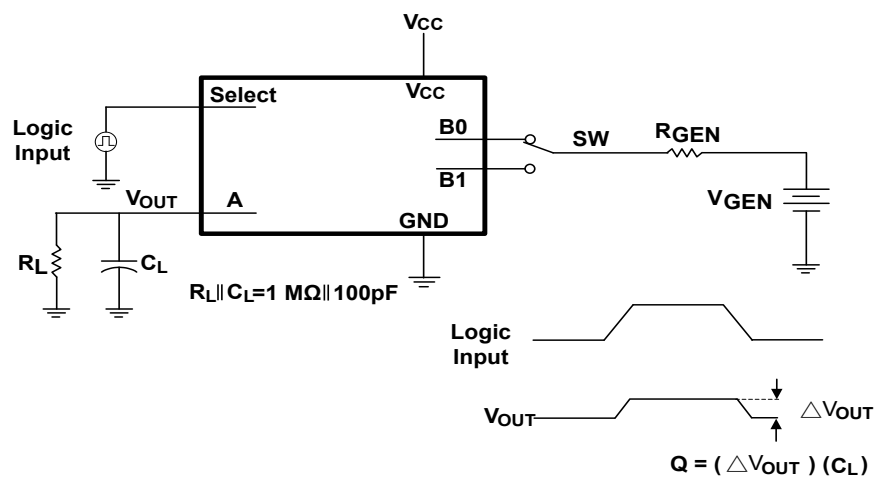
Figure 6 Charge Injection
