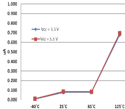
Figure 25 I_{S(ON)} ON state leakage V_{IN} = -0.1 V
