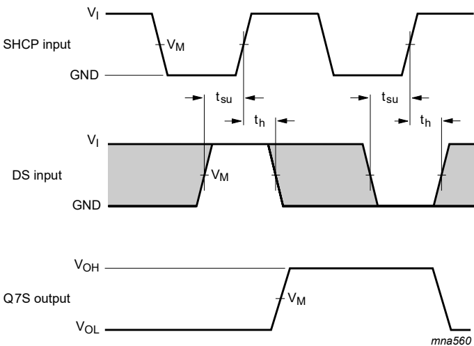
Measurement points are given in Table 16 . V_{OL} and V_{OH} are typical output voltage levels that occur with the output load.
