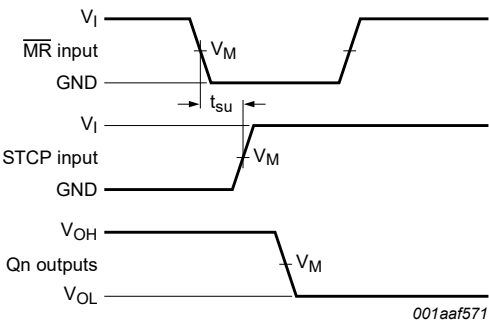
Measurement points are given in Table 16 . V_{OL} and V_{OH} are typical output voltage levels that occur with the output load.
