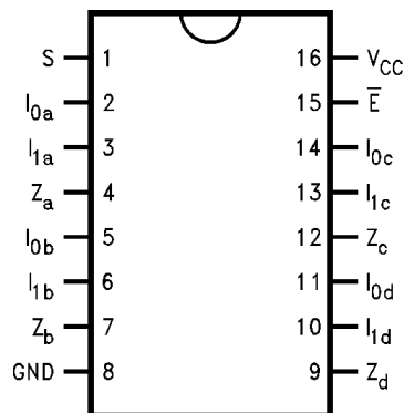
Figure 1. Connection Diagram
