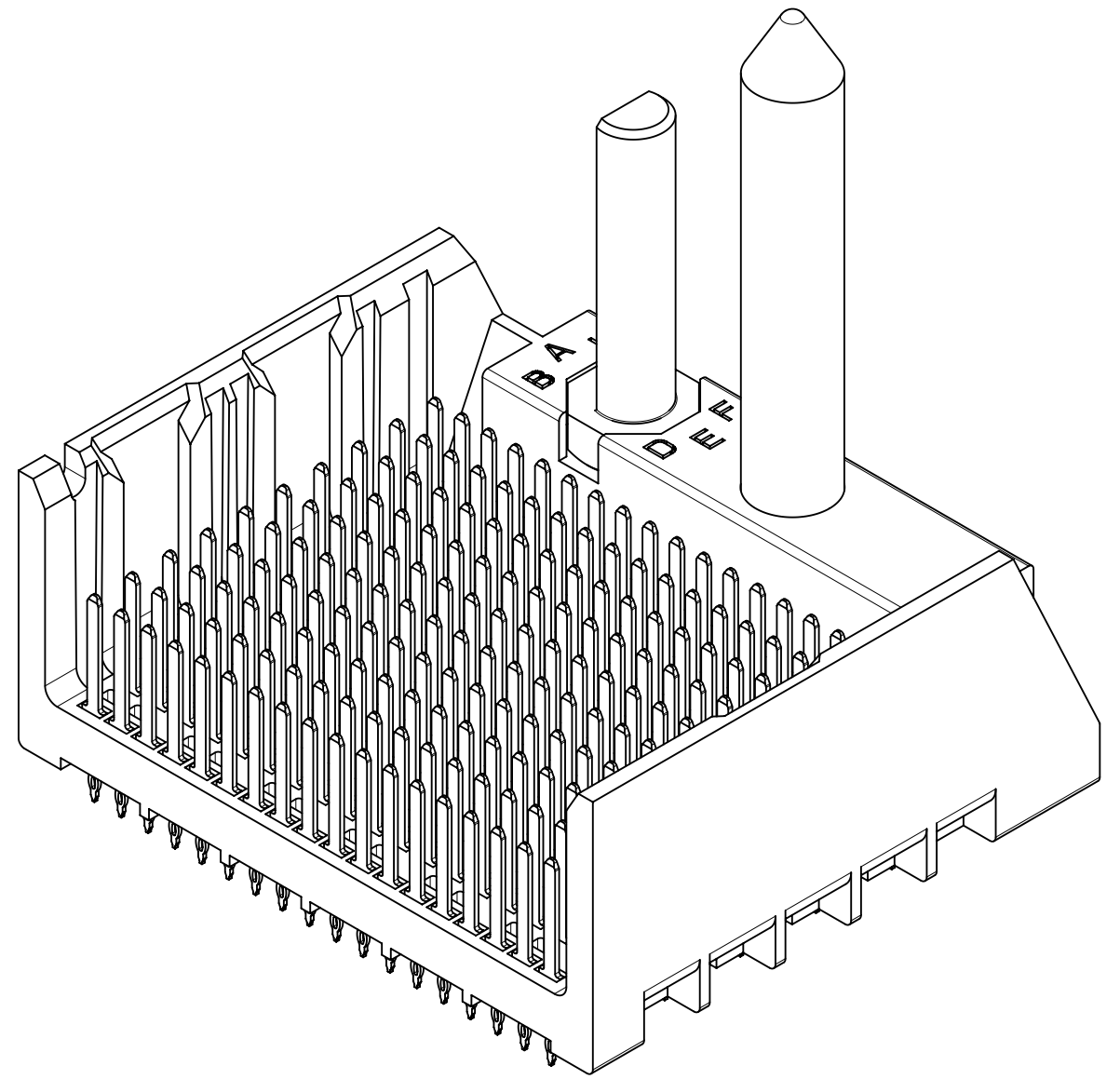
GUIDE RIGHT OPEN WALL OPTION
