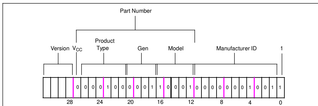
Figure 40. 80960JD Device Identification Register Fields
