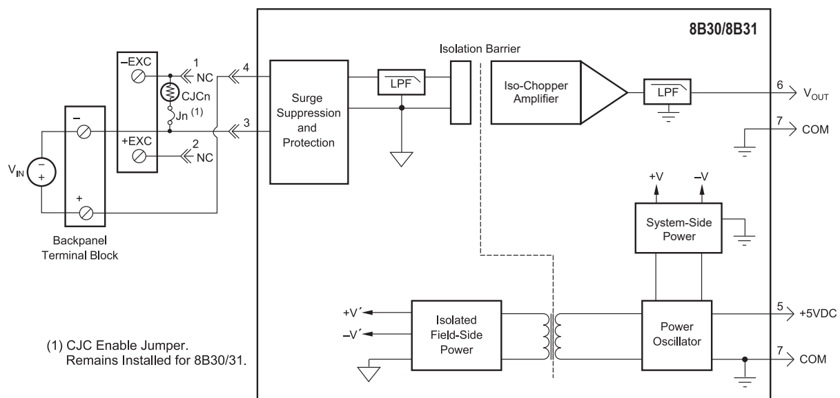
8B30/31 Block Diagram - For Module Dimensions and Pinouts, See Page 3-40
