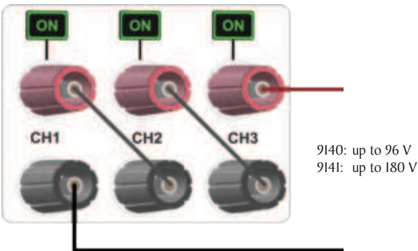
Series mode increases voltage
