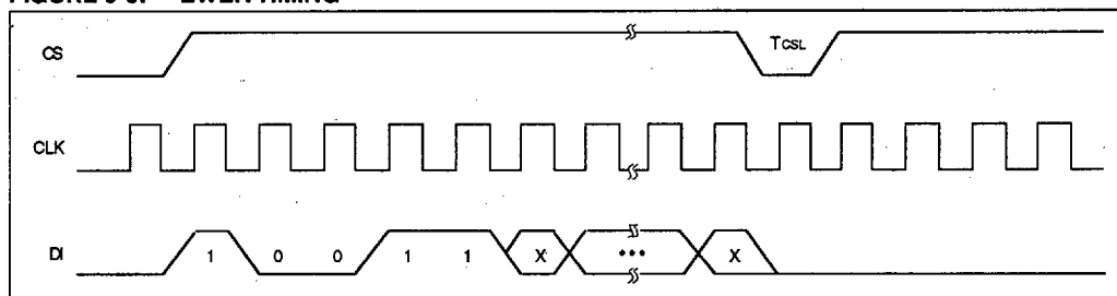
FIGURE 9-3: EWEN TIMING
