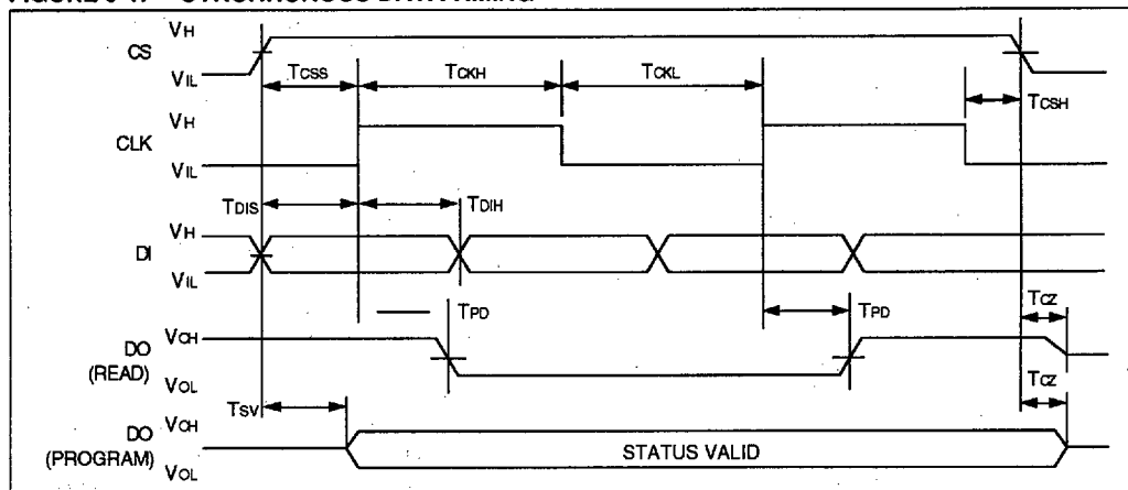
FIGURE 9-2: READ TIMING
