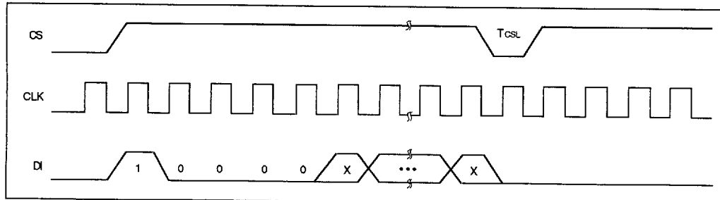
FIGURE 9-5: WRITE TIMING
