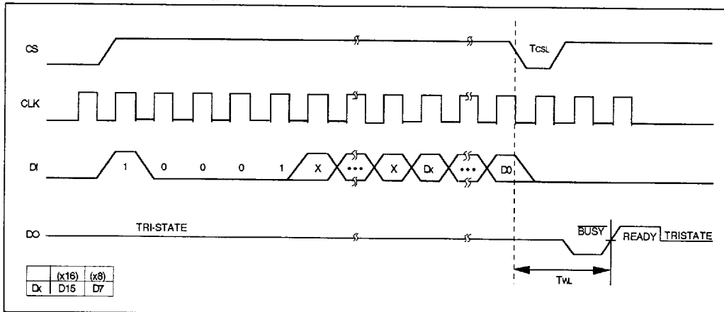
FIGURE 9-6: WRAL TIMING
